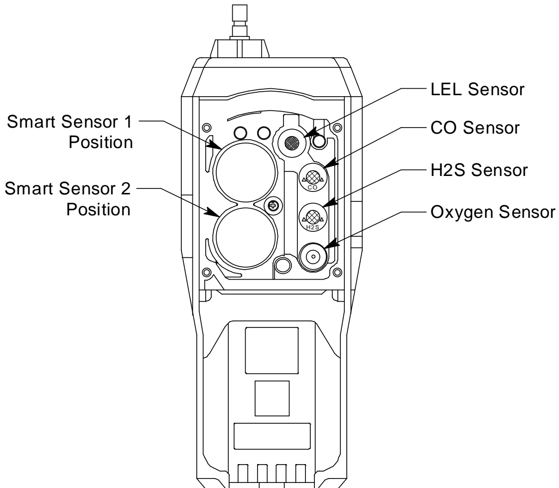
Figure 37: Sensor Location Diagram
