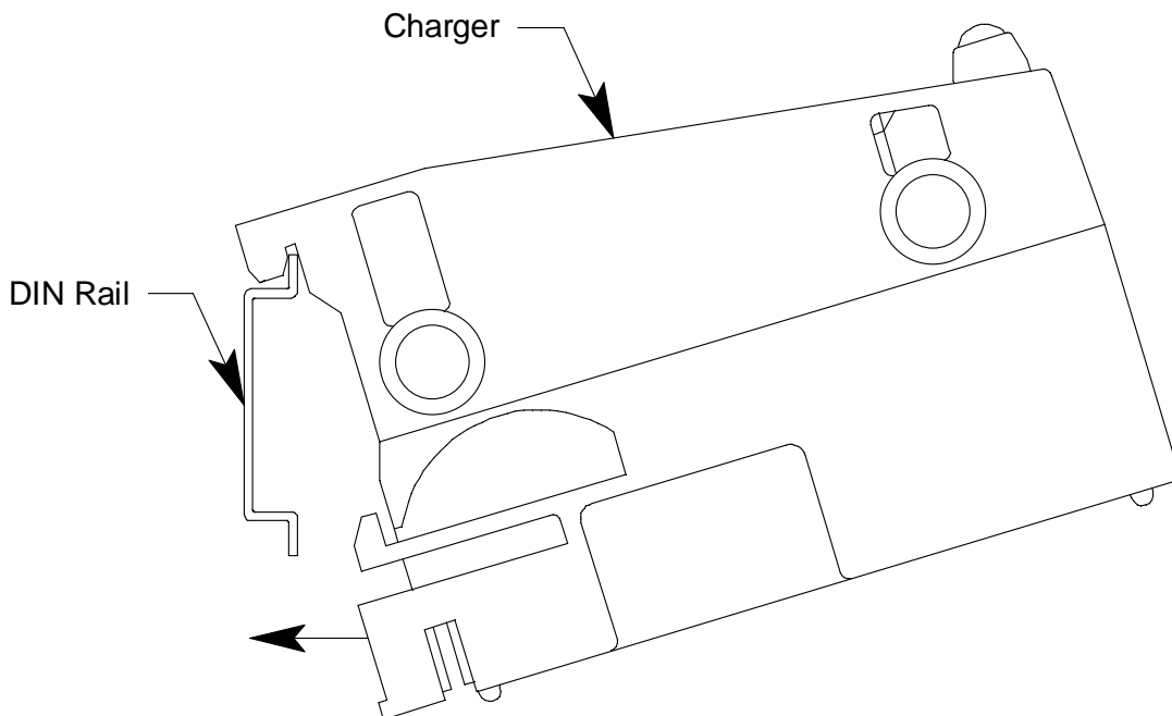
Figure 6: Installing a Charger on the DIN Rail
