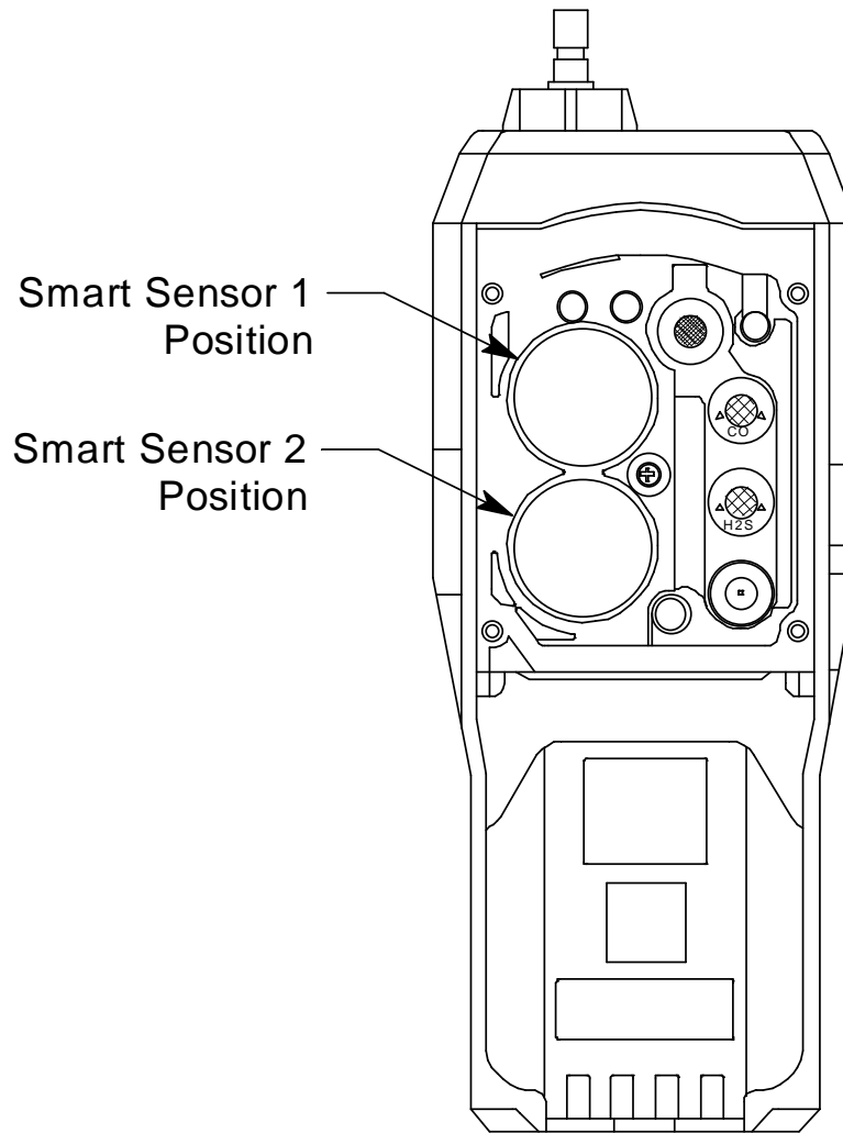
Figure 34: Smart Sensor Positions
