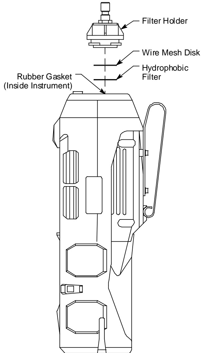
Figure 25: Changing the Filter & Wire Mesh Disk
