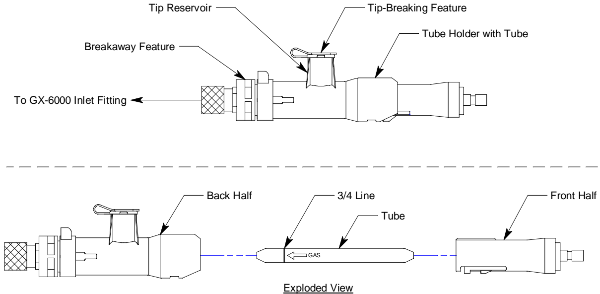
Figure 38: Tube Holder Component Location
