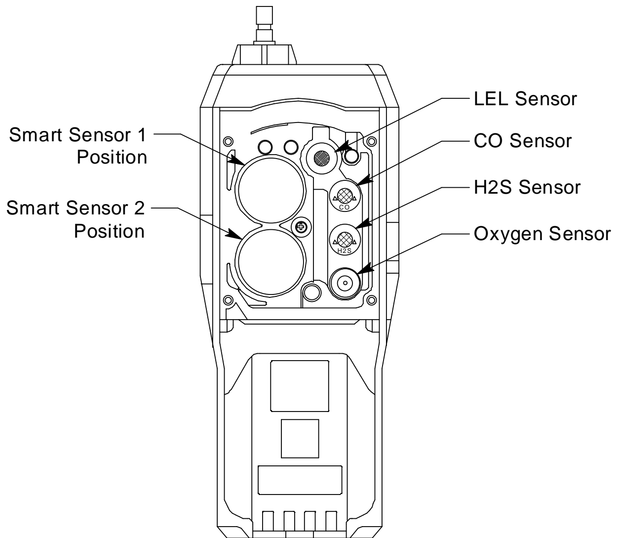
Figure 24: Replacing a Sensor
