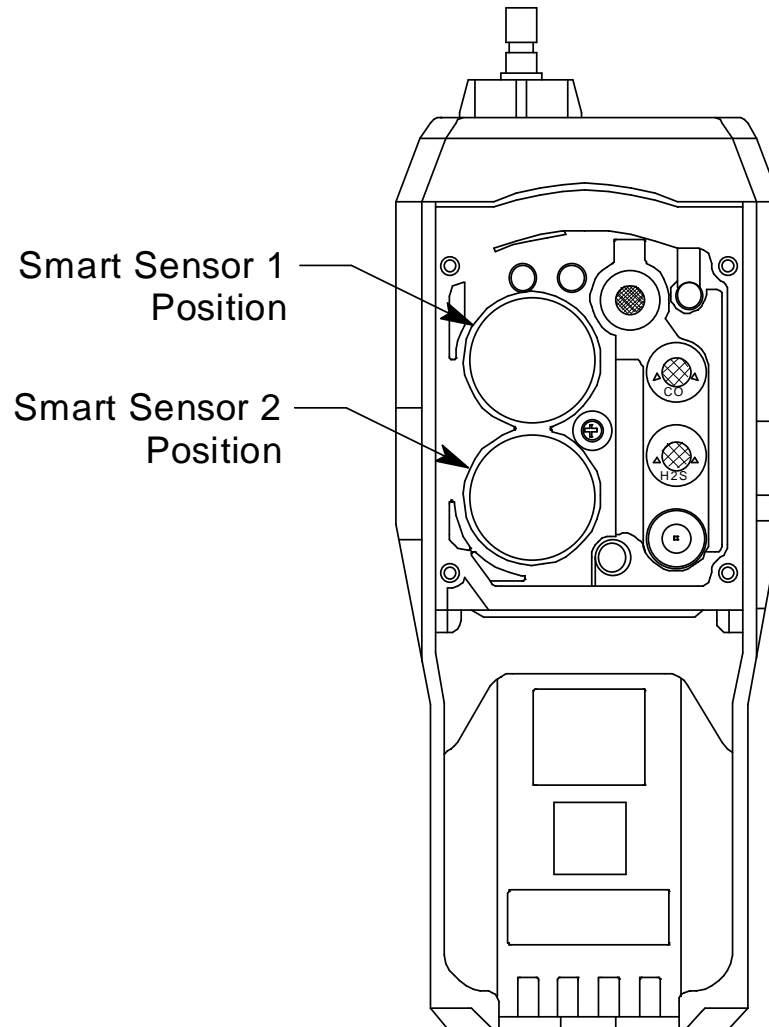
Figure 36: Smart Sensor Positions
