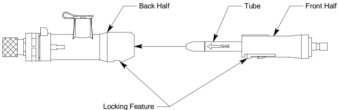
Figure 41: Reassembling Tube Holder
