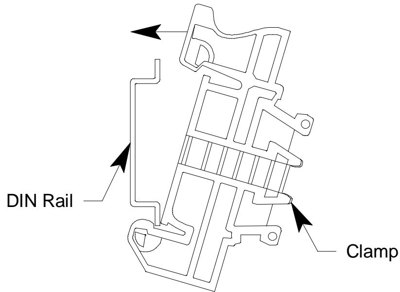
Figure 7: Clamp Installation
